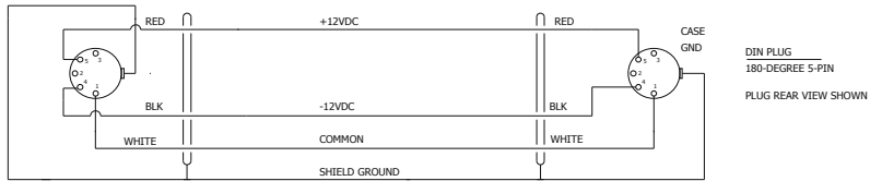
LC 0737 POWER INTERCONNECT CABLE
