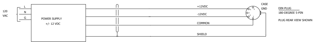
LD 0741 POWER SUPPLY & CABLE
