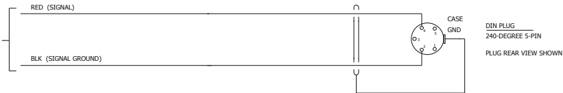
LC 0732 SIGNAL CABLE
