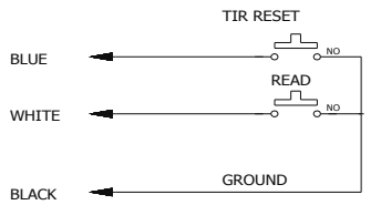
PUSHBUTTON WIRING
