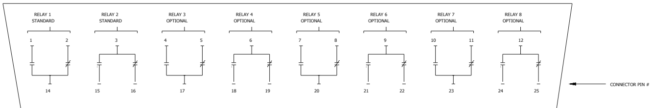
25-PIN SUBMINERATURE 'D' CONNECTOR - FEMALE
